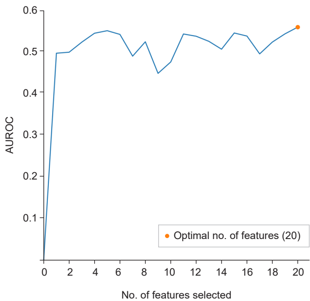
Fig. S1. Area under the receiver operating characteristic curve (AUROC) based on selected variables.
